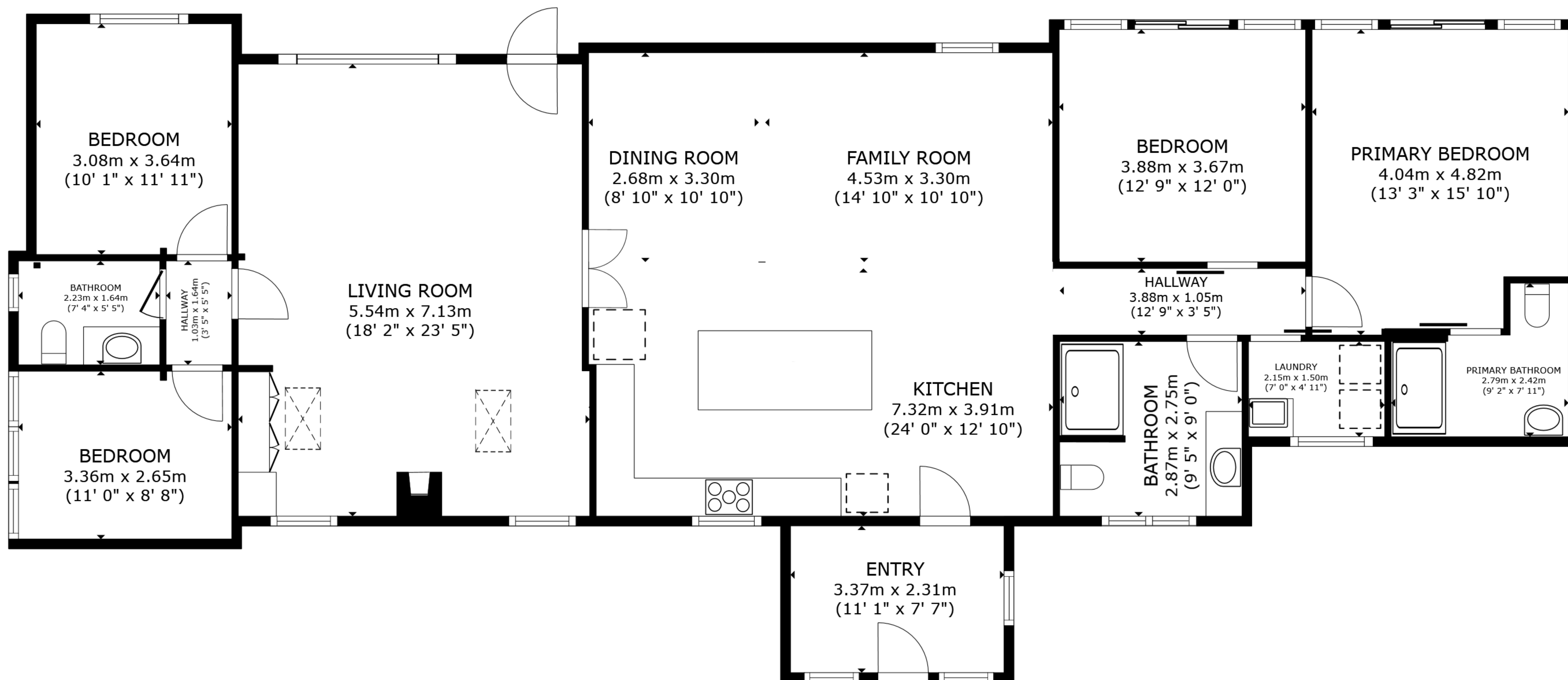
FLOOR PLAN
